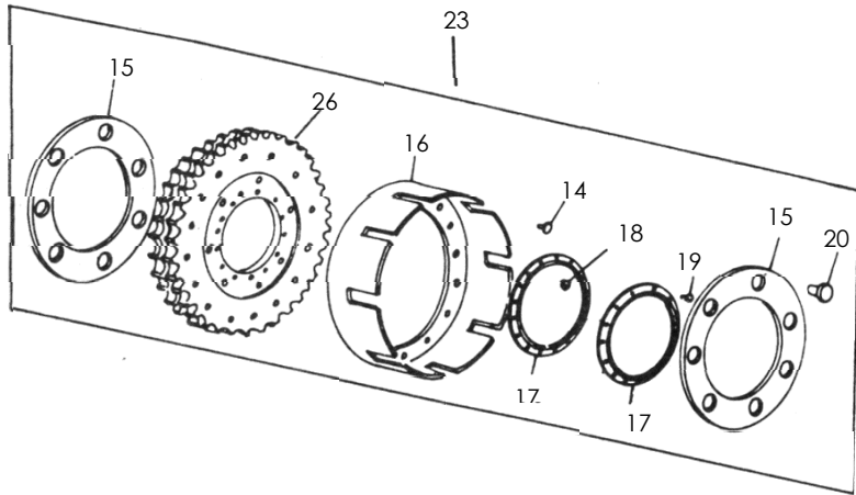
Four Speed Gear Box
